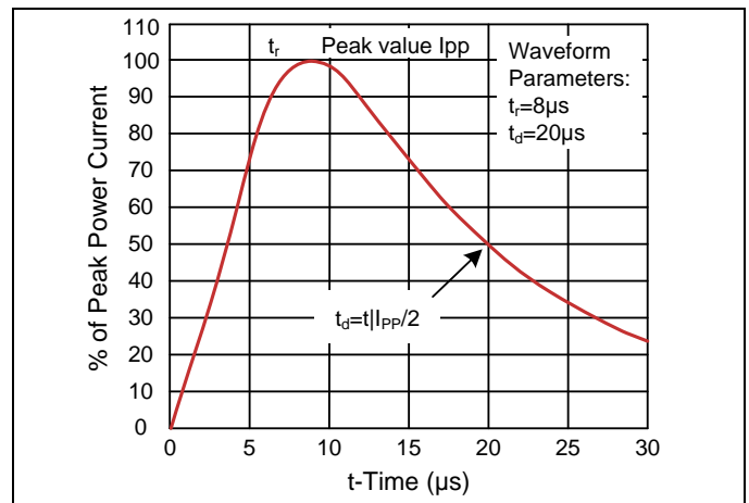
Figure 2. Pulse Waveforms
