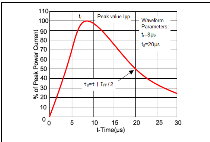
Figure 1. Pulse Waveforms
